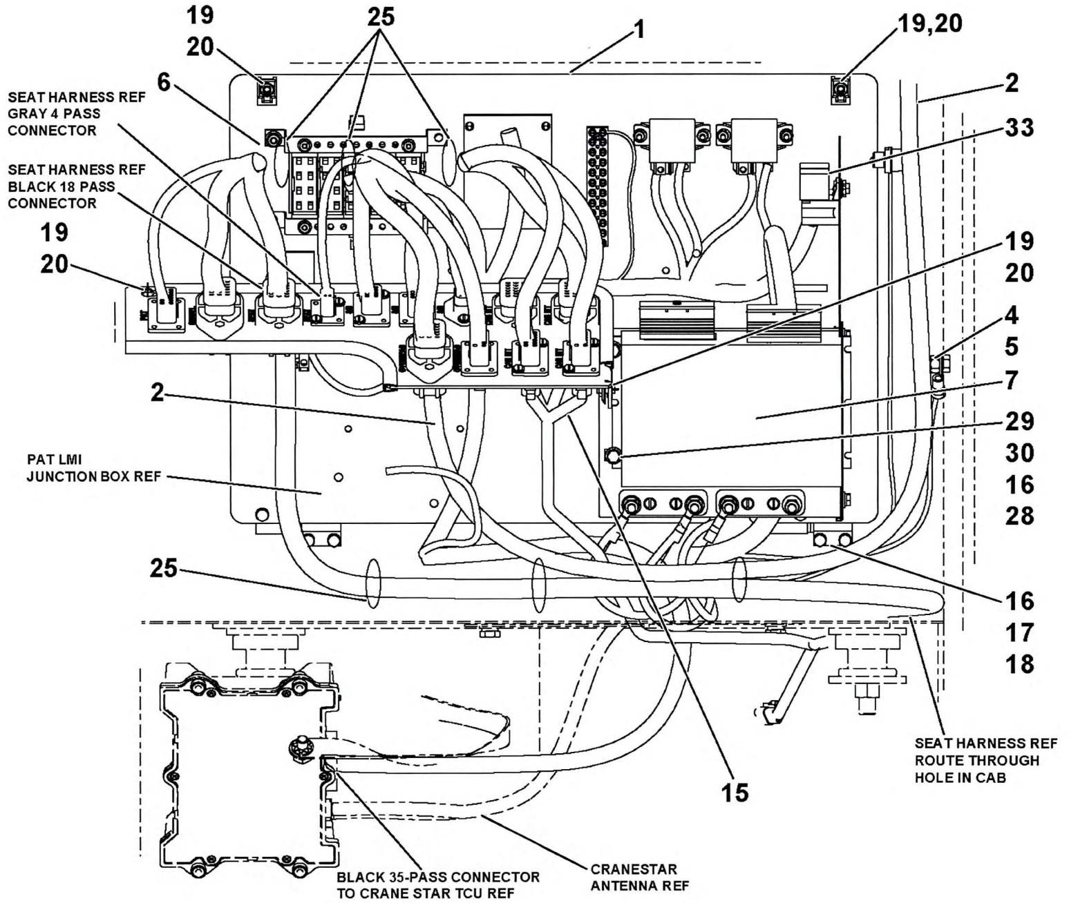
DETAIL-K FUSE & RELAY PANEL
